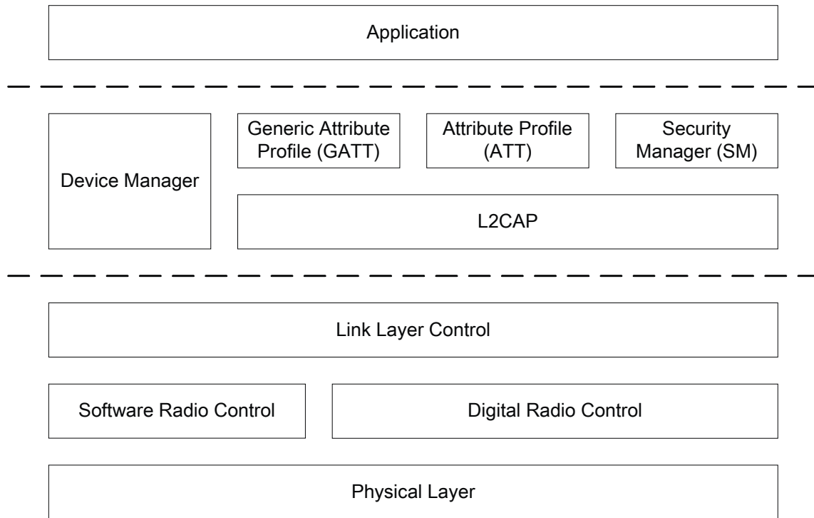
Figure 11.1: Software Architecture
