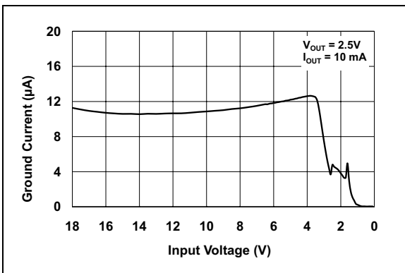
FIGURE 2-33: Ground Current vs. Input Voltage.
