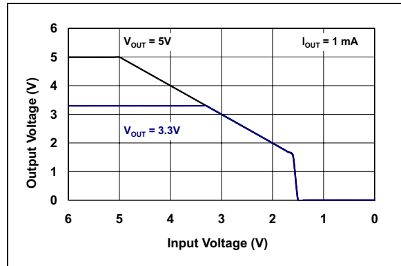
FIGURE 2-35: Output Voltage vs. Input Voltage.
