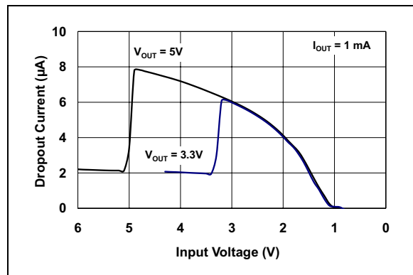
FIGURE 2-36: Dropout Current vs. Input Voltage.
