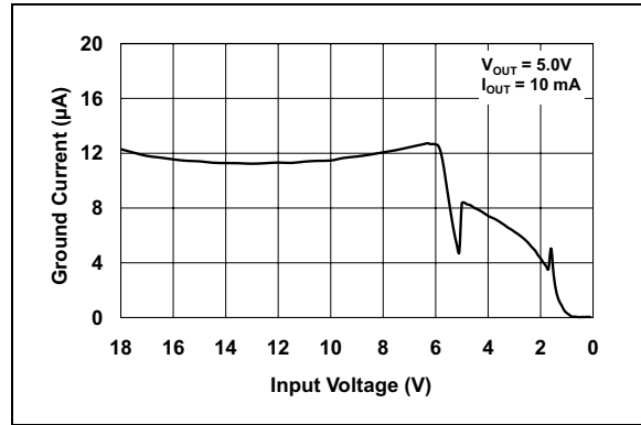
FIGURE 2-34: Ground Current vs. Input Voltage.
