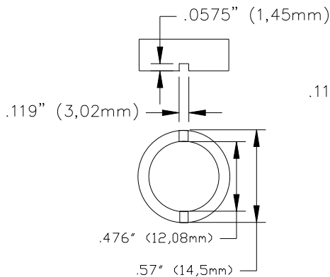
PANEL CUTOUT
