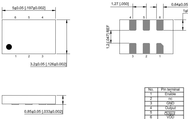
External Dimensions
