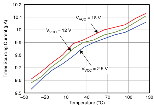
Figure 26. Timer Sourcing Current vs Temperature at Various Input Voltages
