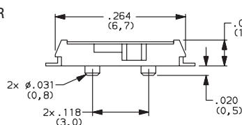
PCM12SMTR SPDT
