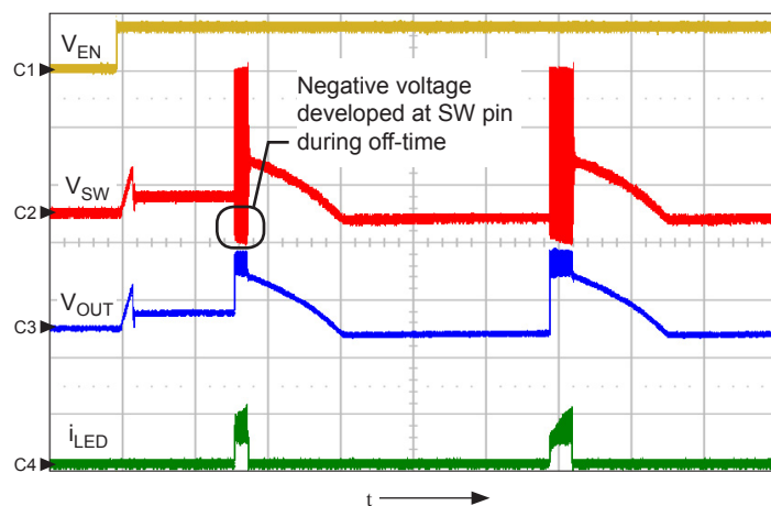
Figure 11: Startup waveform with a missing Schottky diode; shows Enable, V_{EN} (ch1, 5 V/div.), switch node, V_{SW} (ch2, 5 V/div.), output voltage, V_{OUT} (ch3, 5 V/div.), LED current, i_{LED} (ch4, 500 mA/div.), t = 100 \mu s/div.
