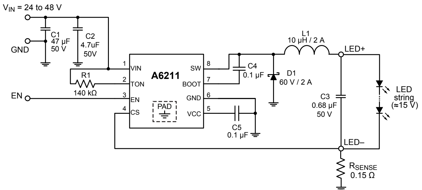
Figure 15: Application circuit diagram
