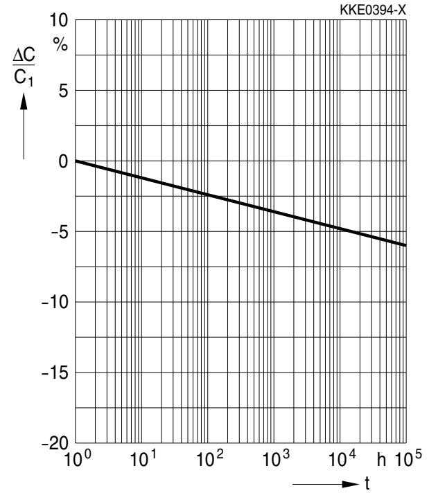
Capacitance change \Delta C/C_1 versus time t
