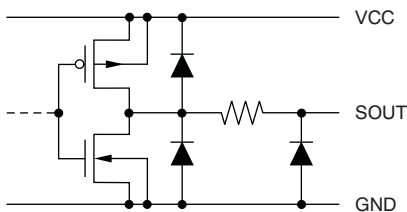
Figure 3. GSSOUT, DCSSOUT
