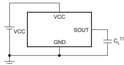
Figure 6. Rise Time and Fall Time Test Circuit for GSSOUT and DCSSOUT
