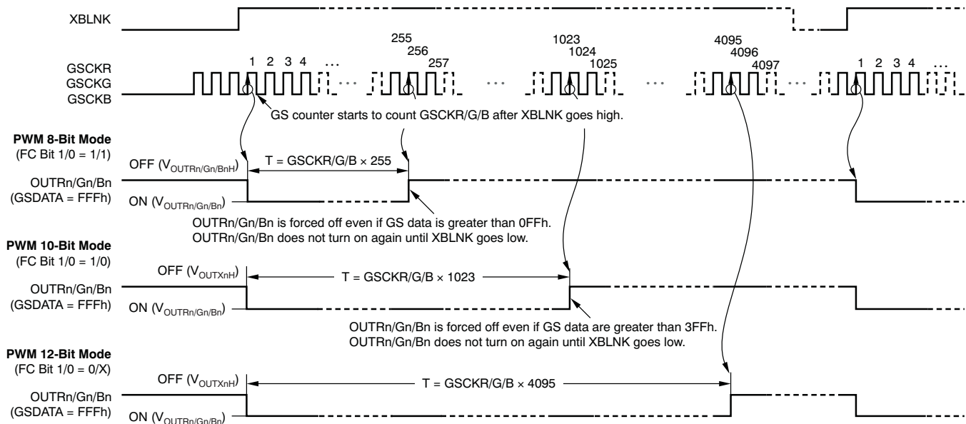
Figure 42. PWM Operation 2
