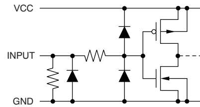
Figure 2. GSSIN, XBLNK
