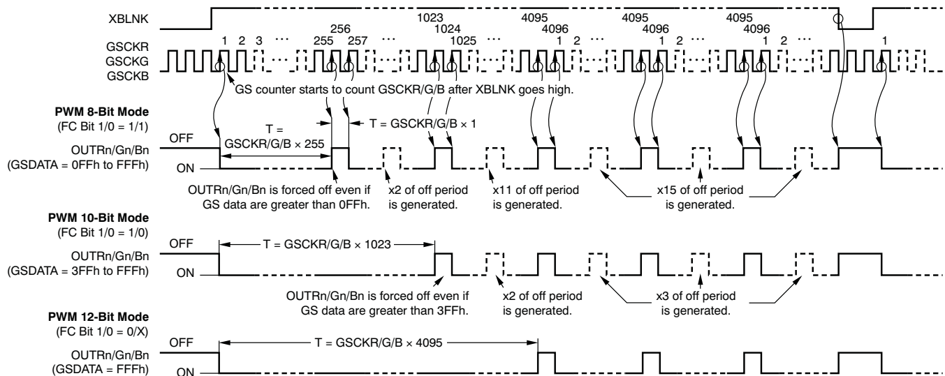
Figure 43. PWM Operation 3
