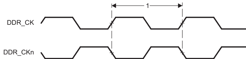
Figure 5-37. DDR2 Memory Interface Clock Timing
