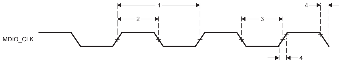
Figure 5-3. MDIO_CLK Timing
