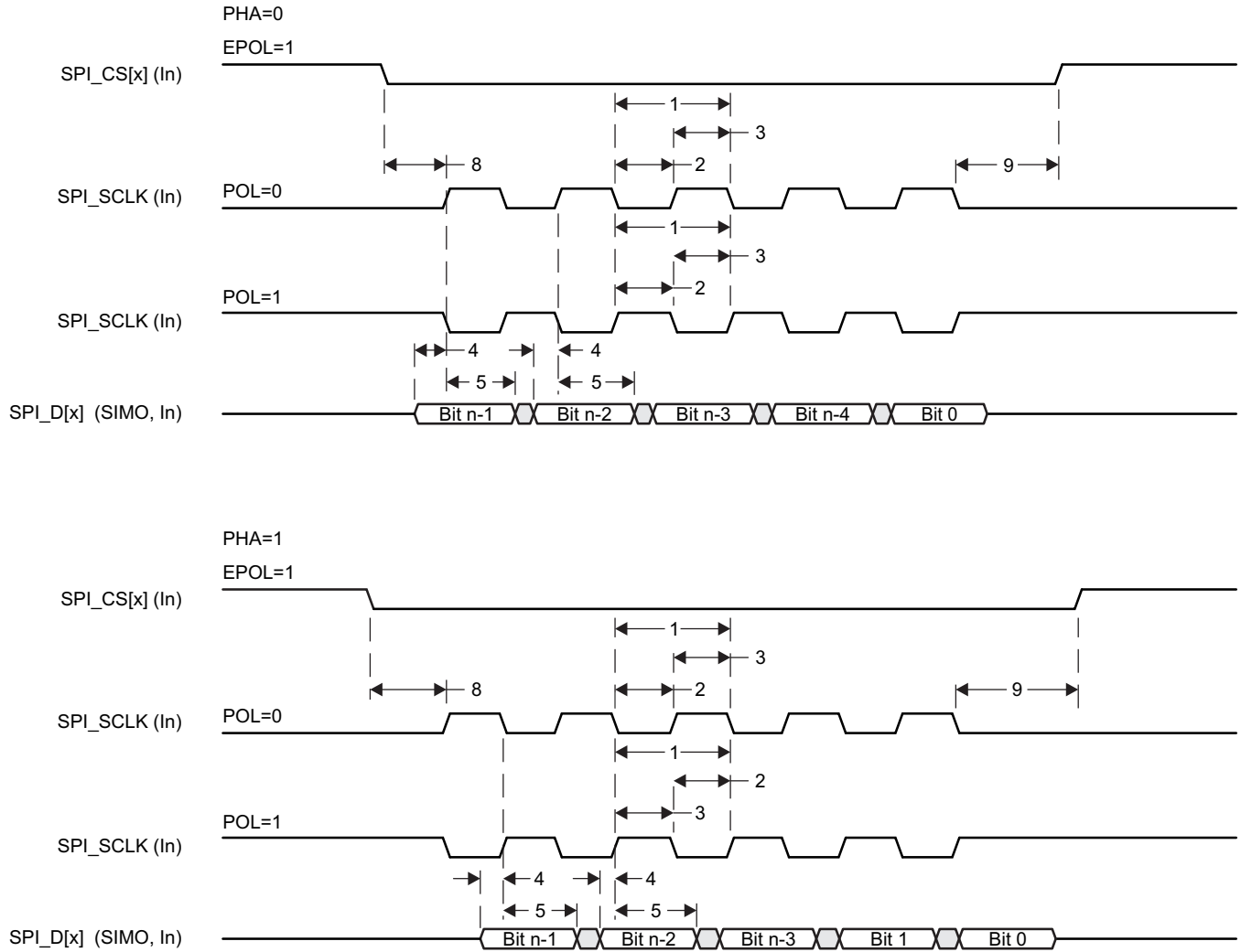
Figure 5-86. SPI Slave Mode Receive Timing
