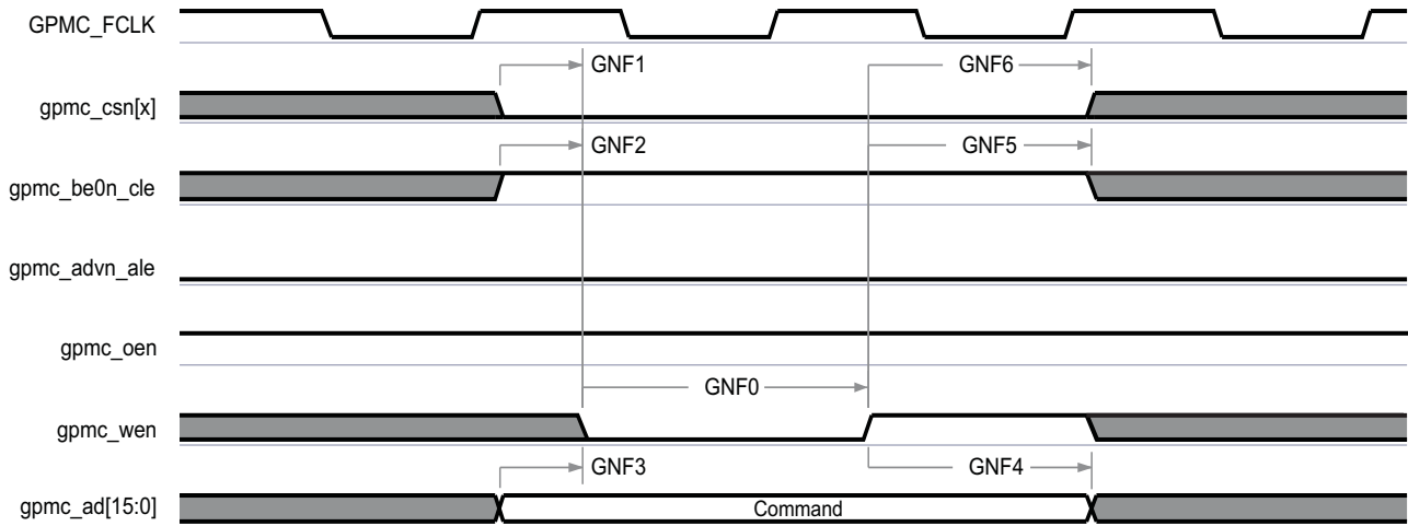
Figure 5-27. GPMC and NAND Flash—Command Latch Cycle
