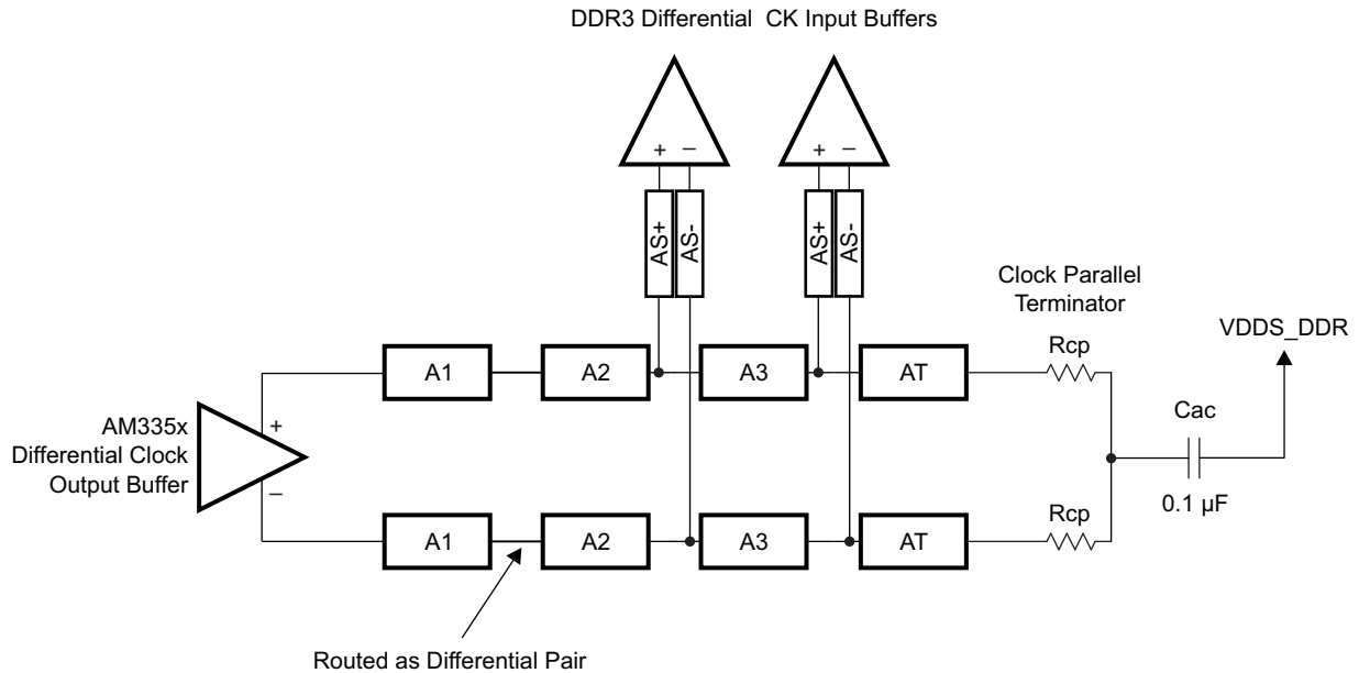
Figure 5-51. CK Topology for Two DDR3 Devices
