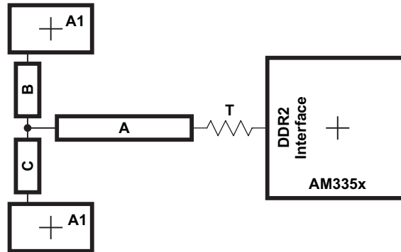
Figure 5-43. CK and ADDR_CTRL Routing and Topology
