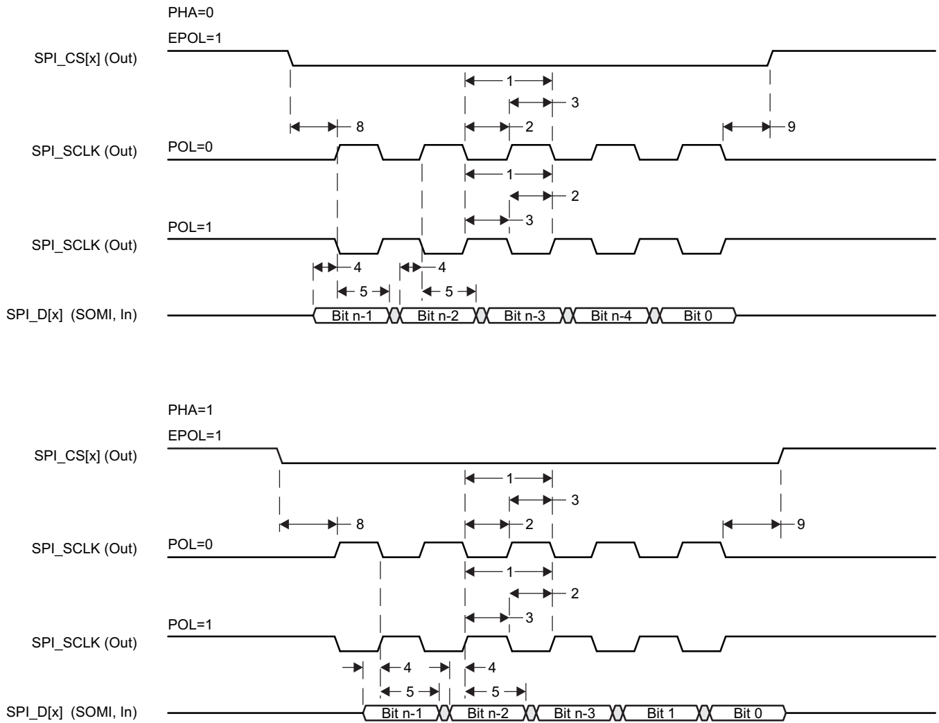
Figure 5-88. SPI Master Mode Receive Timing
