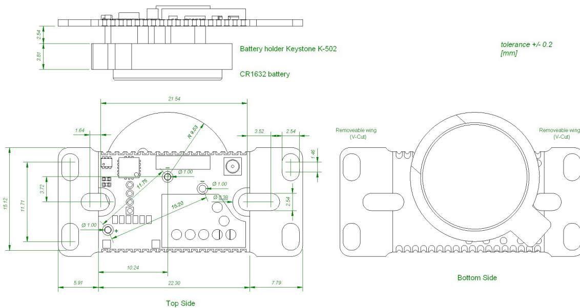
Figure 12: cB-OLP425 dimensions with mounting wings (optional, on request only) and CR1632 battery holder.
