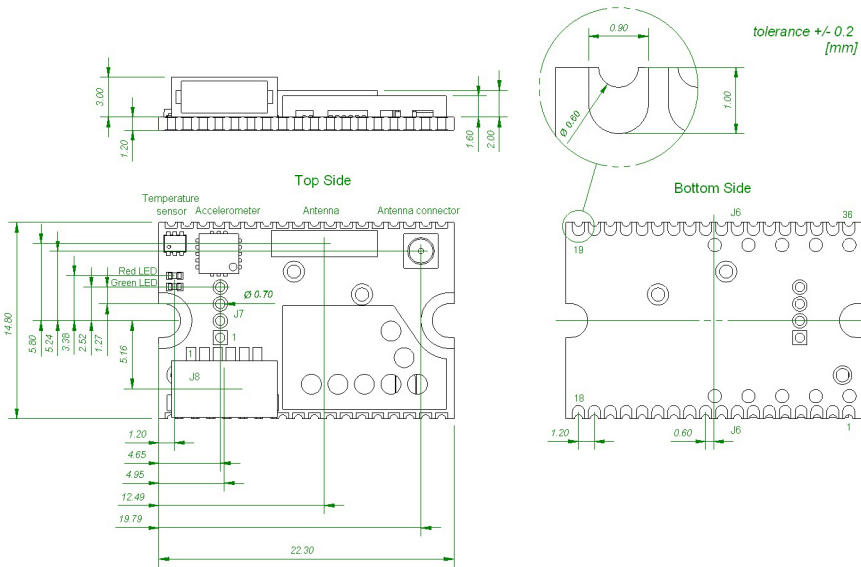
Figure 11: cB-OLP425 and cB-OLS425 module dimensions.
