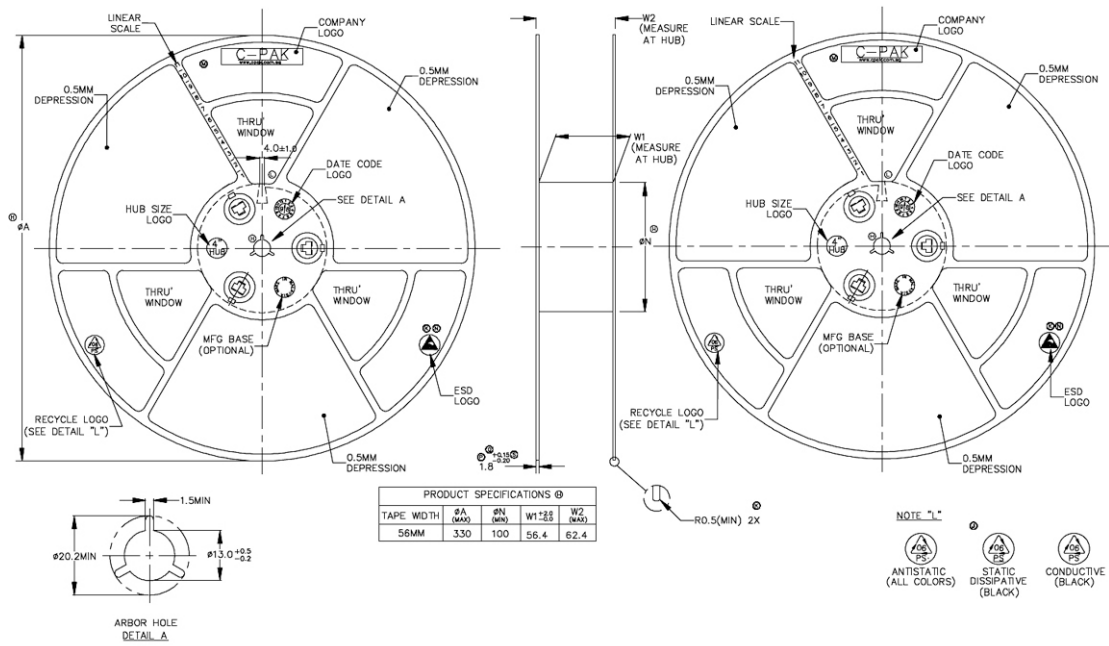
Figure 18: Tape reel dimensions.
