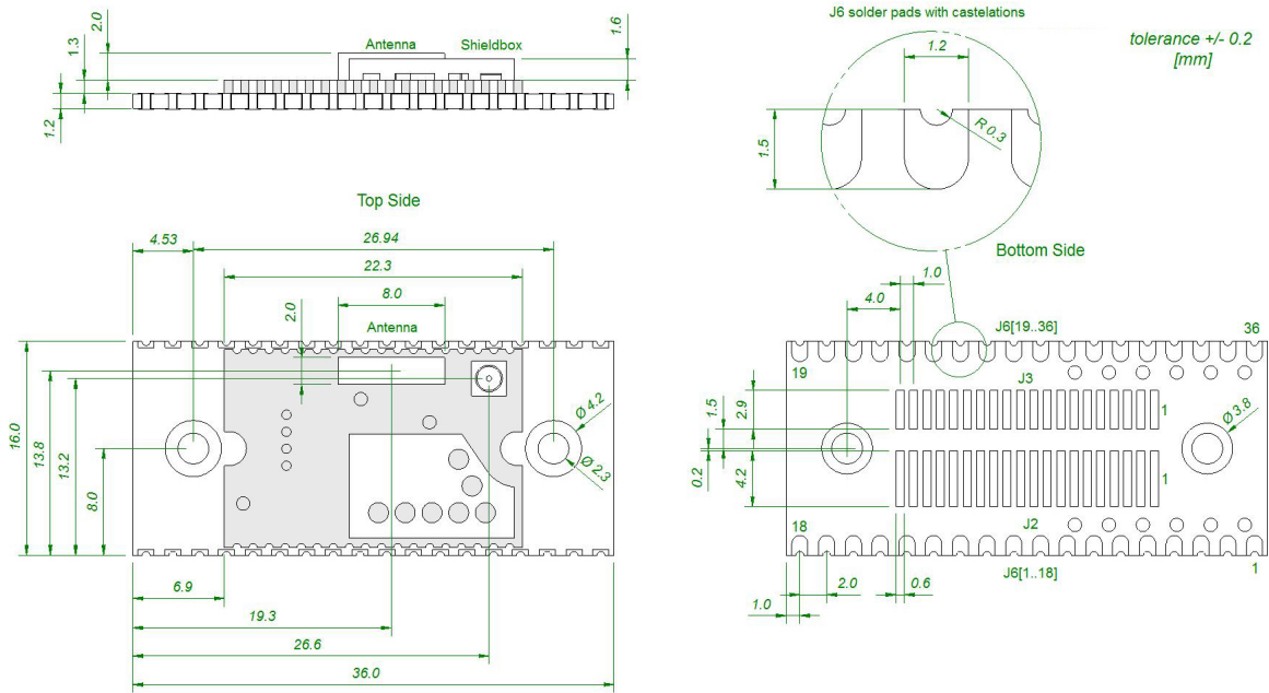
Figure 13: cB-OLS426 dimensions.
